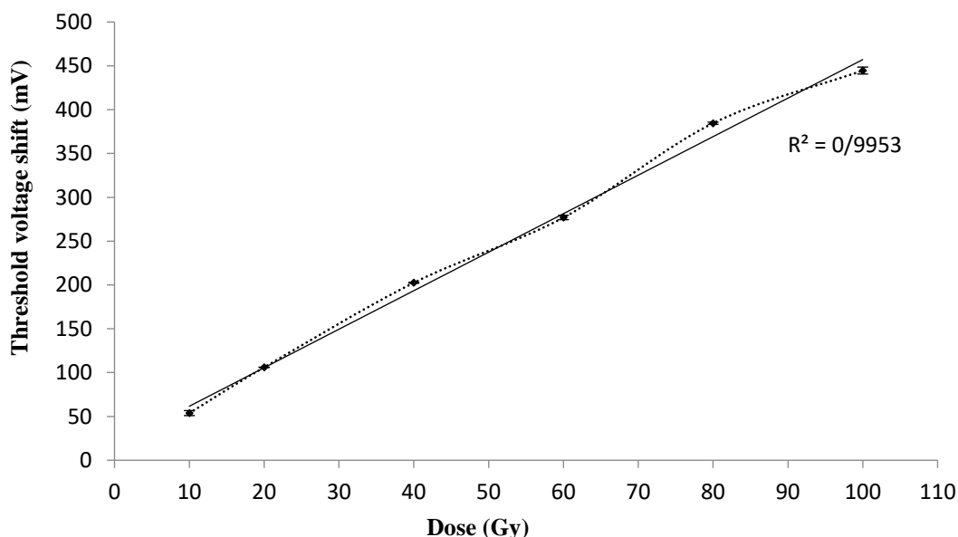
Fig. 4. The Threshold voltage changes of CD4007 transistor in different doses up to 100 Gy Fig. 5. shows the angular dependence of CD4007 transistor that was irradiated at dose of 5 Gy. The orientation of the normal line on the sample page with the incident gamma-ray was assumed as the measurement angle and set at \theta = \pm 60^\circ and the average photocurrents were measured. The results show a change of 0.5% of the photocurrent in comparison to the response obtained at \theta = zero.
