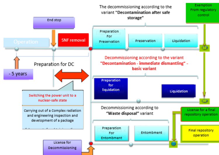
Fig. 7. Diagram of the NPP decommissioning Options/Strategies
