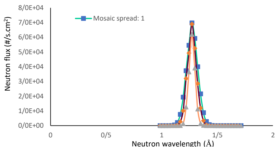
Fig.11. Vitess output for the reflected neutrons from PG(002) crystal with 11^\circ glancing angle and reflectivity of 1.
