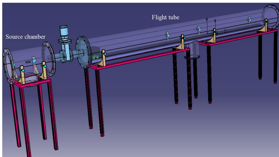
Fig. 2. Structure of the A-TOF spectrometer under construction at the Nuclear Science and Technology Research Institute.
