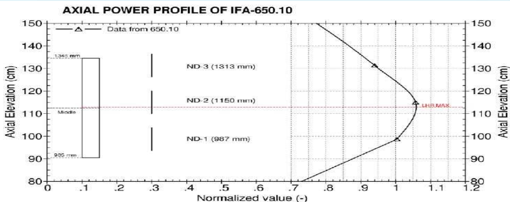
Fig. 6. Axial power profile at the start of the test of IFA-650.10 [13]
