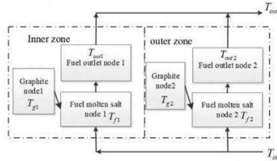
Fig. 1. Division of liquid molten salt reactor core
