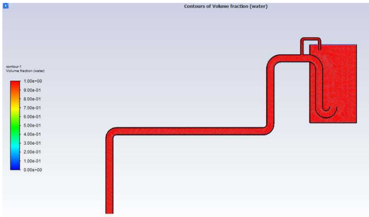
Fig. 2. The geometry used in the simulations.
