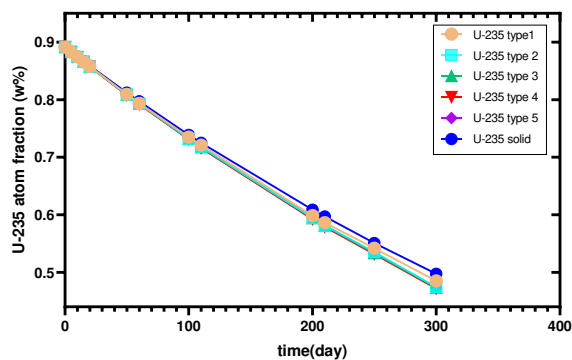
Fig 7. U-235 depletion versus time operation.
