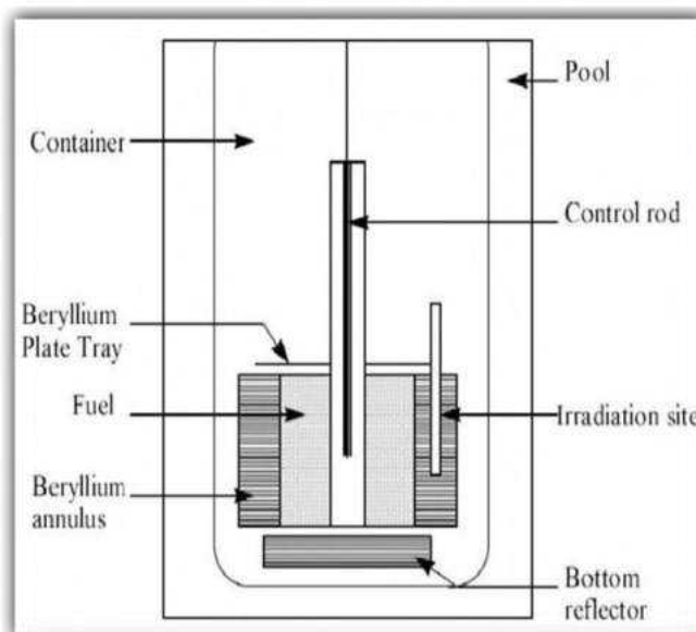
Fig.1. A schematic of the MNSR.
