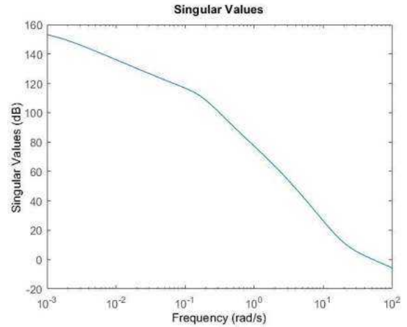
Fig. 4. Singular values after applying the integrator
