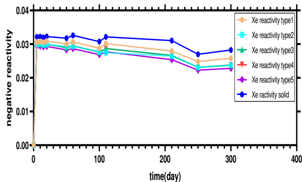
Fig 10. Negative reactivity due to Xe-135 production.
