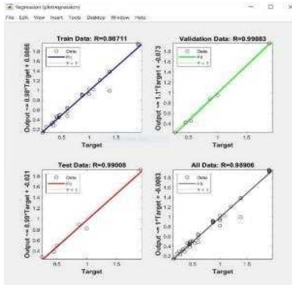
Fig.10. Neural Network Training Regression
