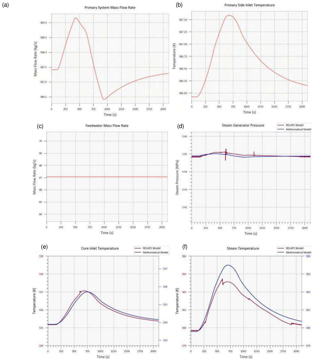
Fig. 5. System response to transients in primary parameters.
