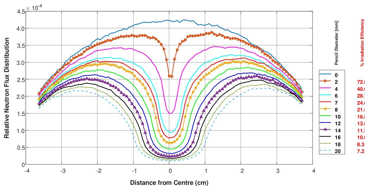
Fig. 2 Relative thermal neutron flux distribution for different diameters of Cobalt-59 pencils in D5 irradiation position.
