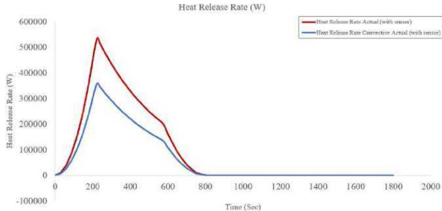
Figure 6: Heat release rate in the presence of an standard fire alarm and extinguishing system
