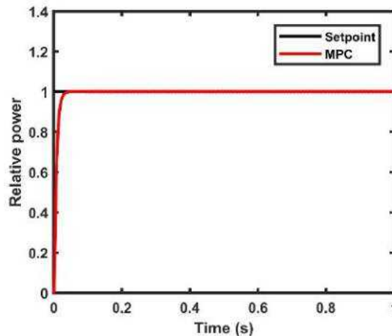
Fig. 6. Controller comparison
