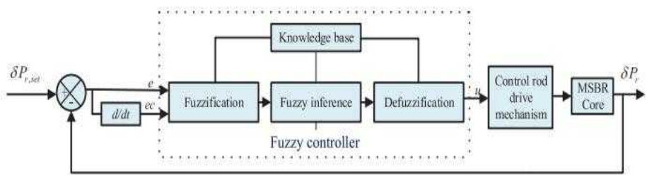
Fig. 3. Fuzzy control block diagram
