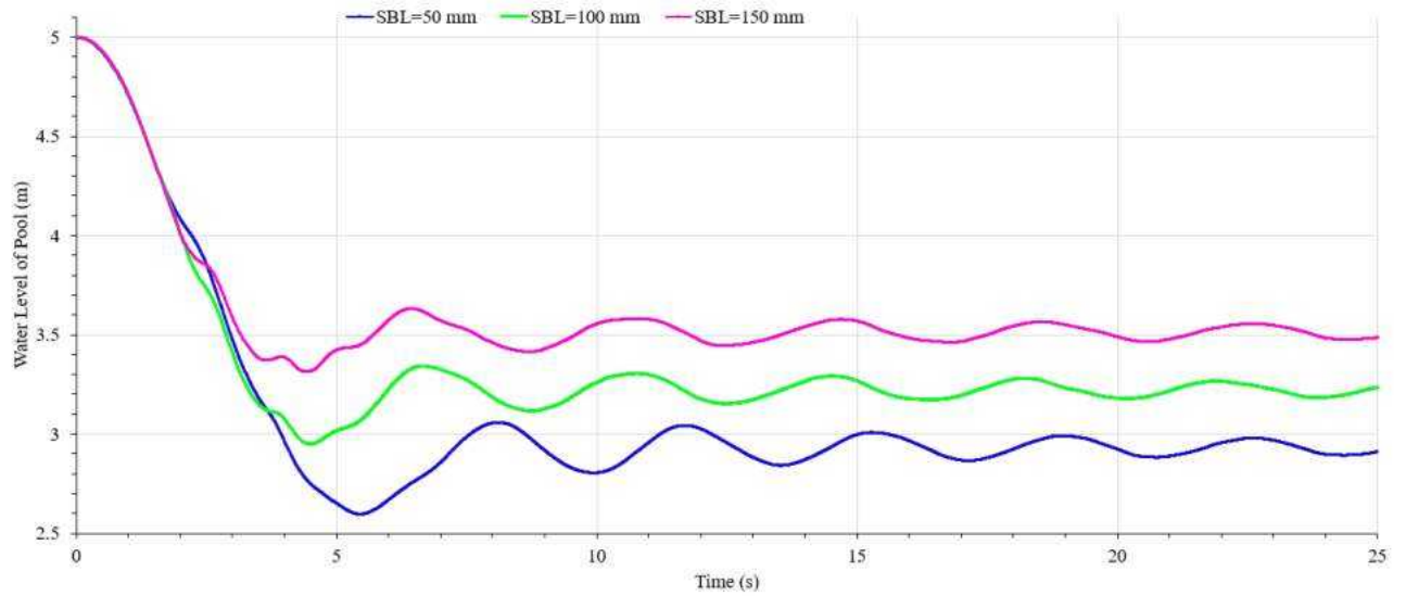
Fig. 4. Pool water level for the SBL sizes of 50, 100, and 150 mm.
