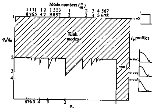
Fig. 6.7.2 Stability diagram for kink modes for the current distributions j = j_0(1 - (r/a)^2)^{\nu} . The vertical axis measures the peaking of the current as given by q_0/q_0 (= \nu + 1) and the horizontal coordinate is proportional to 1/q_0 and therefore to the total current.
