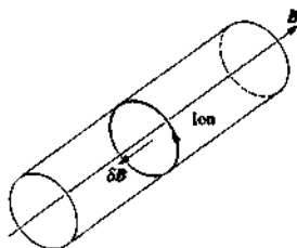
Fig. 2.22.1 Ions with a given velocity having Larmor orbits on a cylinder produce a magnetic field \delta B inside the cylinder, this field being in the opposite direction to the total magnetic field B .
