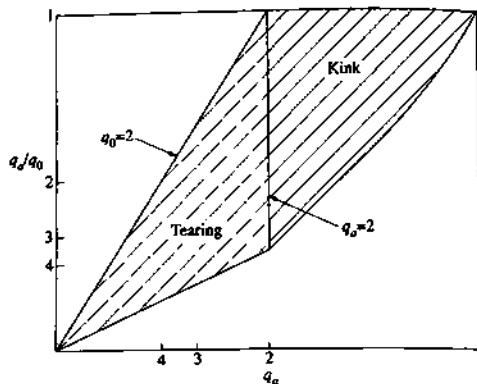
Fig. 6.9.2 Stability diagram for the m = 2 kink and tearing modes for current distributions j = j_0(1 - (r^2/a^2))^p . Stability for q_0 > 2 results from the absence of a resonant ( q = 2 ) surface.
