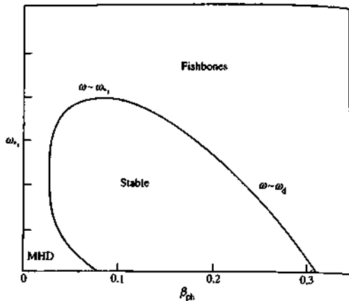
Fig. 7.14.2 Stability diagram in the (\omega, \beta_{ph}) plane where \beta_{ph} is the poloidal beta of the hot particles. Outside the stable region there is the fishbone instability, with the real frequencies indicated, and the MHD m = 1 kink mode which appears at small \beta_{ph} . (From Coppi, B. et al. , Physical Review Letters 63, 2733 (1969).)
