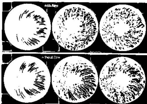
Fig. 4.21.2 Turbulence simulations with a gyrokinetic code, the turbulence evolving in time from left to right. The behaviour with sheared flow is shown in the upper panel, the initial linear, radially extended structures being broken up by the flow. The lower panel shows the behaviour without sheared flow and the extended structures are seen to persist into the non-linear regime. (Lin, Z. and Tang, W.M. Physics of Plasmas 9, 1856 (2002).)
