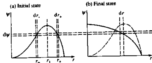
Fig. 7.6.6 Mapping of the flux from the initial state to the final state in Kadomtsev's model of the sawtooth collapse.
