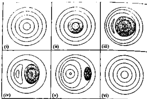
Fig. 7.6.4 Development of the magnetic field structure during the sawtooth instability according to Kadomtsev's model (following Sykes, A. and Wesson, J.A., Physical Review Letters 37, 140 (1976)). The m = 1 instability displaces the q < 1 region (shown shaded) and restores q to a value > 1 .
