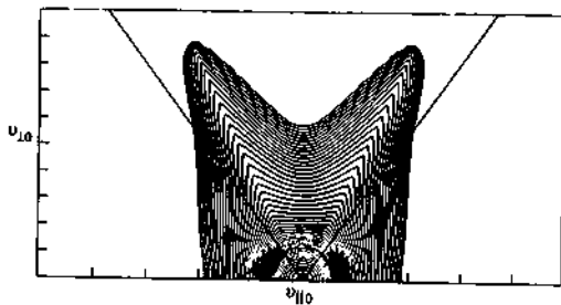
Fig. 5.8.8 Contours of the steady state ion distribution represented in midplane velocity space coordinates ( v_{\perp 0} , v_{\parallel 0} ) for a minority ion excited at its second harmonic cyclotron frequency. The oblique lines mark the trapped-passing boundary and both figures show the accumulation of heated ions which turn flame their banana (ps) in the resonance region. A similar result has also been obtained for fundamental ion cyclotron resonance of minority ions. [From Kerbel, G.D. and McCoy, M.G., Physics of Fluids 28, 3269 (1985).]
