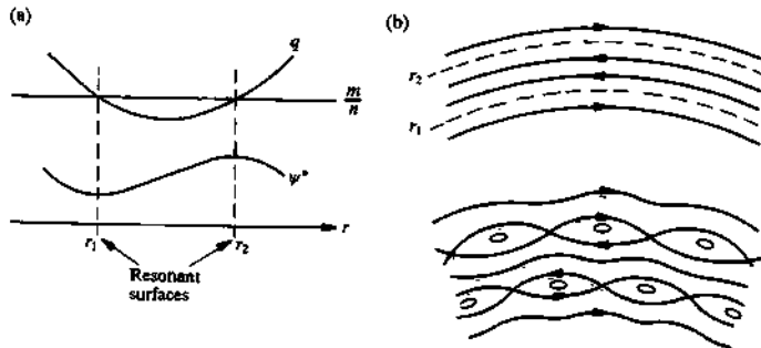
Fig. 7.5.2 (a) A minimum in q allows two resonant surfaces with the same values of m and n . \psi^* is the corresponding helical flux. (b) The two resonant surfaces lead to two sets of magnetic islands.
