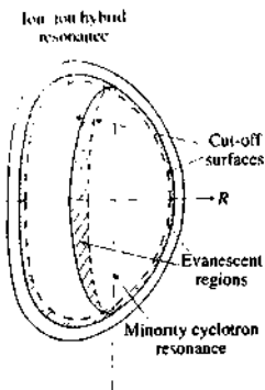
Fig. 5.8.1 Loci of cut-off and resonances in the poloidal cross-section of a tokamak. The fast wave is evanescent in the hatched regions.
