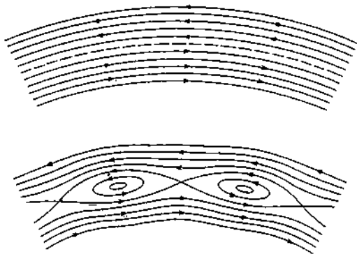
Fig. 7.2.1 Reconnection of magnetic field producing magnetic islands.
