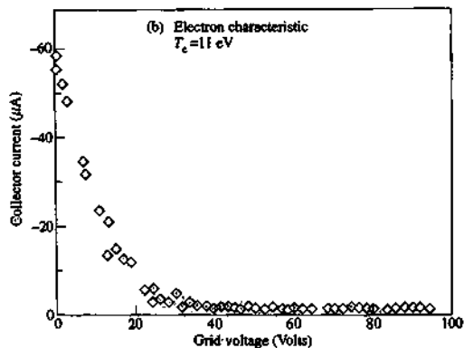
Fig. 9.2.2 Integral energy distributions measured in the plasma boundary of the DITE tokamak (a) ions, (b) electrons. (Pitts, R.A. Physics of Fluids 3, 2871 (1991).)
