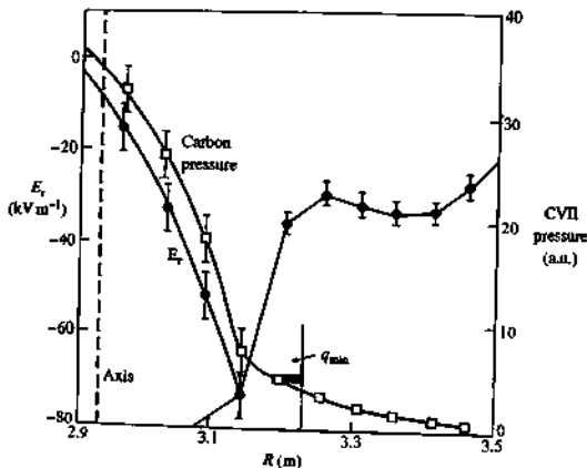
Fig. 4.14.2 Radial electric field and carbon pressure profiles in an BRS discharge in TFTR. Fluctuations and turbulent fluxes are reduced inside the transport barrier near the minimum in q . Correspondingly, the carbon pressure profile has a steeper gradient in this region. The transport barrier is associated with a rapidly varying profile of E_r .
