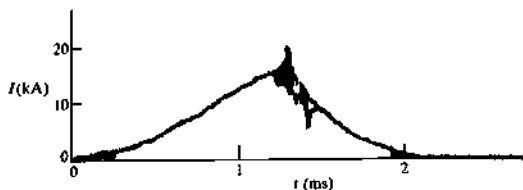
Fig. 7.1.3 Early experimental observation of current collapse brought about by a plasma disruption (Gorbanov, E.P. and Razumova, K.A. Plasma Physics 6, 515 (1964) from Atomnaya Energiya 15, 363 (1963))
