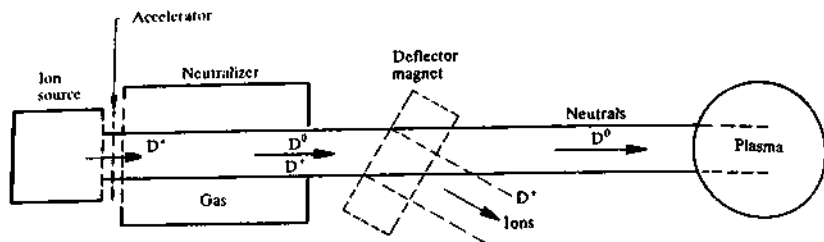
Fig. 6.6.1 Layout of neutral injection system.
