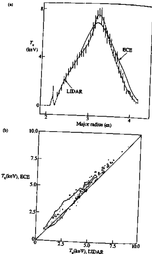
Fig. 10.5.6 Comparison of T_e determined by ECE and LIDAR measurements. Good agreement is found for both (a) the profiles for a particular discharge and (b) the averaged central temperature for a wide range of different discharges. The contour shows the region within which 90% of the measurements lie.
