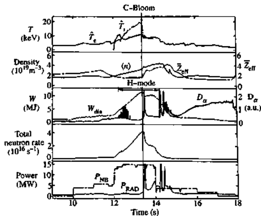
Fig. 12.3.17 The time development of the central electron and ion temperatures, \bar{T}_e and \bar{T}_i , the volume-averaged electron density, \langle n \rangle , the line-averaged \bar{n}_{eH} , the plasma diamagnetic energy, W_{dia} , the D_\alpha emission, the total neutron rate, the NBI power, P_{NB} , and the radiated power, P_{RAD} , for the deuterium pulse with the highest fusion triple product [The JET Team Nuclear Fusion 32, 187 (1992)].
