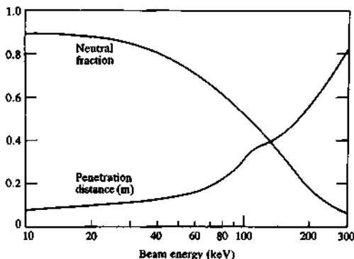
Fig. 5.5.3 Graphs showing the energy dependence of (i) the equilibrium neutral fraction in a deuterium beam and (ii) the penetration distance of the neutrals in a plasma of density n = 10^{20} \text{ m}^{-3} . The change of behaviour of the penetration distance at around 100 keV indicates the transition from charge exchange dominance to ionization dominance.
