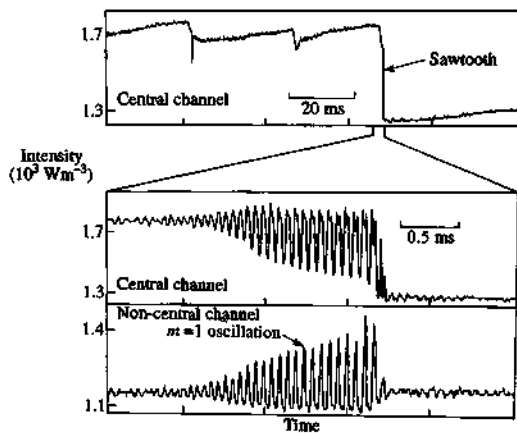
Fig. 10.0.4 Signals from individual detectors of the JET soft X-ray cameras showing a sawtooth in the upper figure and pronounced m=1 activity in the lower figures which are on an expanded timescale. On the rapid timescale the sawtooth precursor activity can be clearly seen both at the plasma centre and at the inversion radius.
