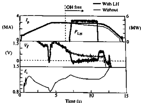
Fig. 12.4.7 Comparison of plasma parameters during two 3 MA plasma pulses, one with full non-inductive current drive using LHCD (dark curve) and the other without LHCD (light curve). The LHCD power, P_{LH} , the plasma current, I_p , the loop voltage, V_L , and the internal inductance, \ell_i , are shown. Note that the ohmic input power is turned off at 6.5 s in both pulses [from Ikeda, Y. et al. Plasma Physics and Controlled Nuclear Fusion Research 1994 (Proc. 15th Int. Conf., Seville, 1994) Vol. 1, 415. I.A.E.A., Vienna (1995)].
