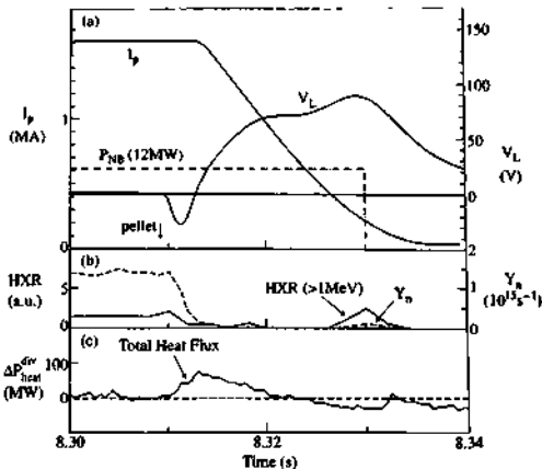
Fig. 12.4.11 Disruptive behaviour following the injection of a cryogenic neon 'killer' pellet: (a) the plasma current, I_p , the loop voltage, V_L , and the NBI heating power, P_{NBI} , (b) hard X-ray, HXR, and neutron yield, Y_n , signals, (c) change in power deposited on the divertor targets, \Delta P_{heat}^{div} [from Yoshino, R. et al. Plasma Physics and Controlled Fusion 39, 313 (1997)].
