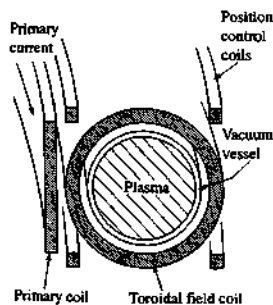
Fig. 1.6.4 Arrangement of coils in a tokamak.
