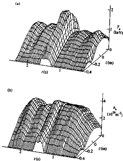
Fig. 10.5.2 Three-dimensional plots of T_e and n_e , during an ASDEX discharge with neutral injection heating applied from 1.3 to 1.6 s. z is the vertical position coordinate. (Röhr, H., Steuer, K.-H., Mürmann, H., and Meisel, D. Proc. of High-Power Solid State Lasers and Applications , Ed. Ireland, C.L.M., SPIE 1277, 154 (1990).)
