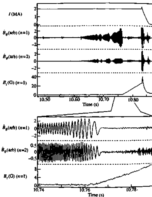
Fig. 7.9.3 An example of the growth of m=1 instabilities in a disruption, with expanded traces around the time of mode-locking. The bottom trace gives the time integrated \dot{B}_t signal, showing the continued instability growth following mode-locking. (Wesson J.A. et al., Nuclear Fusion 29, 641 (1989).)
