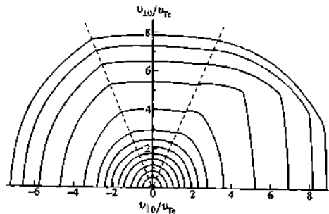
Fig. 5.10.3 Contours of electron distribution function for second-harmonic \lambda_c -mode heating in the COMPASS tokamak for an injected power of 1.5 MW. The other parameters are, n_e = 10^{19} \text{ m}^{-3} , T_e = 1.5 \text{ keV} , f = 60 \text{ GHz} and \rho/R = 0.08 , where \rho is the radius of the resonant flux surface. The dashed lines show the boundaries of trapped and passing electrons. [From O'Brien, M.R., Cox, M., and Stott, D.F.H., Nuclear Fusion 26, 1625 (1986).]
