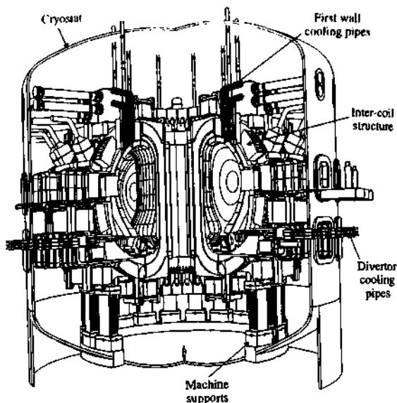
Fig. 13.4.2 Drawing giving an overall view of the layout of Ignition ITER.
