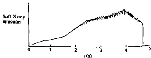
Fig. 7.1.2 Sawtooth oscillations of the soft X-ray emission (JET).
