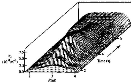
Fig. 10.3.3 Time evolution of the density profile in a pellet fuelled discharge in JET. Each pellet produces a discontinuous increase in plasma density. The first pellet is injected at 2 s and the three subsequent ones lead to a maximum density at about 3.5 s. At later times the density profile broadens.
