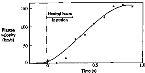
Fig. 3.13.1 Plasma velocity during neutral beam injection as measured by the Doppler shift of the impurity spectral lines (JET).
