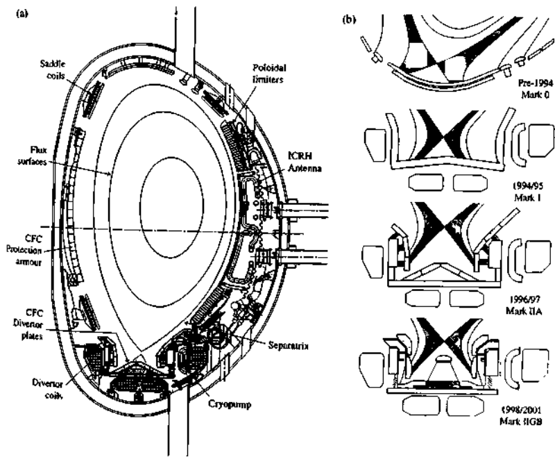
Fig. 12.3.2 (a) Poloidal cross-section of the JET pumped divertor configuration showing the divertor coils, the target plates for the Mark II A configuration and the cryopump. (b) The three principal pumped divertor configurations studied, in chronological order: Mark I, Mark II A, Mark II GB (Gas Box). From 2002 on, experiments were conducted without the central septum dividing the inner and outer divertor legs in the Mark II GB. The original X-point configuration, subsequently referred to as the 'Mark 0', is also shown for comparison.
