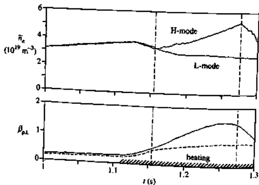
Fig. 4.13.1 Comparison of H- and L-mode discharges with the same heating power. The L-H transition follows the application of tangential neutral beam heating. After the transition the density and the perpendicular component of \beta_p rise to around twice the values reached in the L-mode discharge. (ASDEX team, Nuclear Fusion 29, 1959 (1989).)
