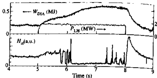
Fig. 12.4.3 Overview of a limiter H-mode induced by LHCD. Shown are the LH power, P_{LH} , the diamagnetic measurement of the plasma stored energy, W_{DIA} , and the H_\alpha emission [from Tsuji, S. et al. Physical Review Letters 64, 1023 (1990)].
