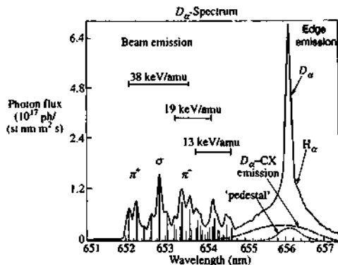
Fig. 10.6.7 Spectrum near the deuterium Balmer-alpha line during beam injection. T_i is found from the broadened feature at about 656 nm. The features at shorter wavelengths are Doppler shifted from the beam. (Wolf, R. et al. , Nuclear Fusion 33, 1835 (1993).)
