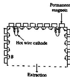
Fig. 5.5.2 Schematic diagram of bucket ion source.
