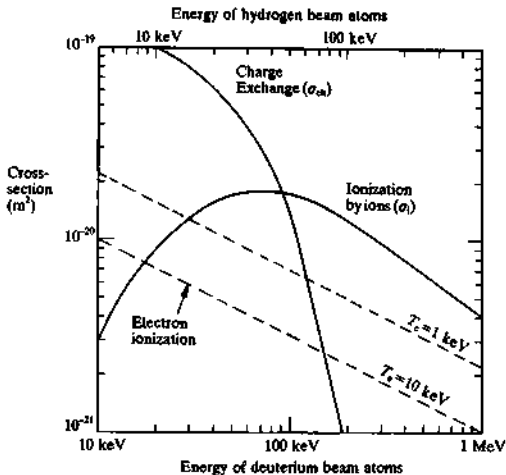
Fig. 5.3.1 Cross-sections for charge exchange and ionization by plasma ions (protons, deuterons, or tritons) and the effective cross-section (\sigma_a N_a)/v_b for ionization by electrons, as functions of the neutral beam energy. The cross-sections for a deuterium beam having twice the energy.
