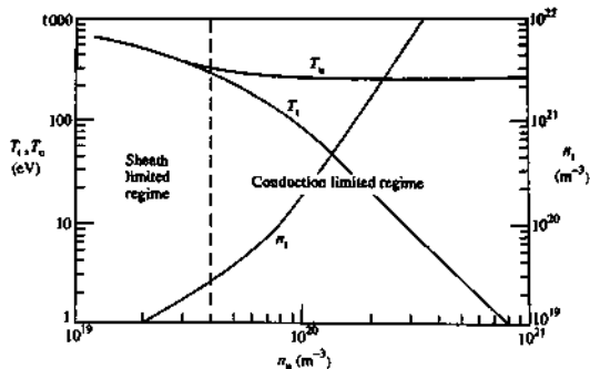
Fig. 9.10.2 Upstream and target temperatures, T_u and T_t , and the target plasma density n_t , as a function of upstream density, n_u , calculated for the one-dimensional model described by eqns 9.10.2, 9.10.4, and 9.10.5. Input power flux q = 1000 \text{ MW m}^{-2} , L = 50 \text{ m} , \gamma_{th} = 10 and ion mass, A = 2 .
