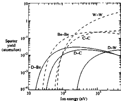
Fig. 9.7.1 Energy dependence of the physical sputtering yield for beryllium, carbon, and tungsten by deuterium and self sputter ions, calculated using a Monte Carlo code. (Eckstein, W. Sputtering data , Report PP9/82 Max Planck Institut für Plasmaphysik Garching, 1993.)
