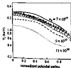
Fig. 12.6.7 H-mode ion temperature profiles measured during a density scan (lines) and for on- and off-axis heat deposition (symbols) are stiff with a constant temperature gradient length T_i/\nabla T_i in the confinement region between 0.3 and 0.8 of normalized poloidal radius.
