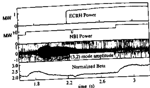
Fig. 12.6.10 Stabilization of neoclassical tearing modes with electron cyclotron current drive as indicated by the amplitude of the m = 3, n = 2 magnetic perturbations. \beta_N = 2.6 was achieved in steady state without these modes by raising the neutral beam power.
