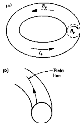
Fig. 1.6.1 (a) Toroidal magnetic field B_t and poloidal magnetic field B_p due to toroidal current I_p . (b) Combination of B_t and B_p causes field lines to twist around plasma.
