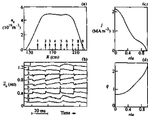
Fig. 10.3.5 (a) Profile of electron density across major radius. (b) Measured fluctuating part of n_e at different radii. (c) Deduced current density profile. (d) Safety factor profile. The data was taken for a sawtooth discharge in TEXTOR. (Soltwisch, H. et al. , Plasma Physics and Controlled Nuclear Fusion Research (Kyoto) 1, 263. IAEA (1987).)
