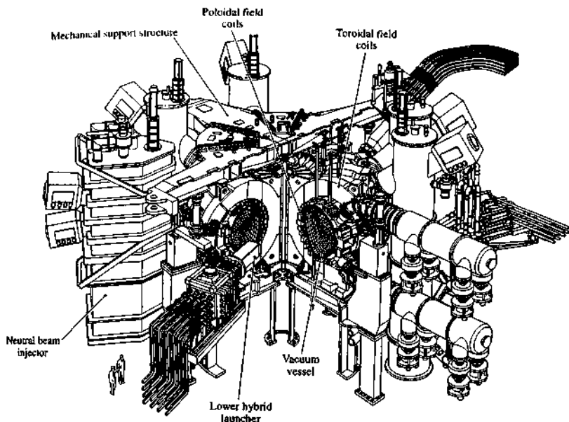
Fig. 12.4.2 Layout of the JT-60U experiment.
