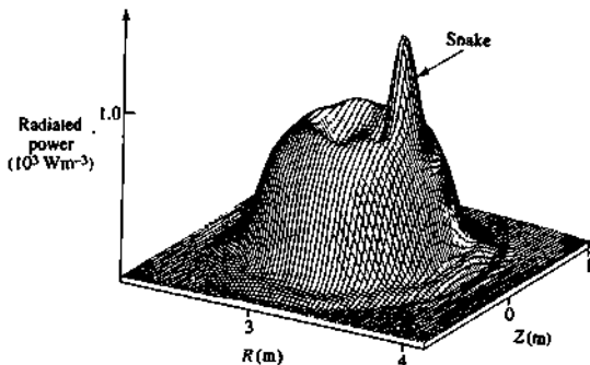
Fig. 10.8.7 Tomographic reconstruction of the snake which is a small region of enhanced plasma density in JET produced on the q = 1 magnetic surface following injection of a solid D_2 pellet.
