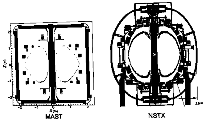
Fig. 11.19.2 Cross-sectional drawings of MAST and NSTX.
