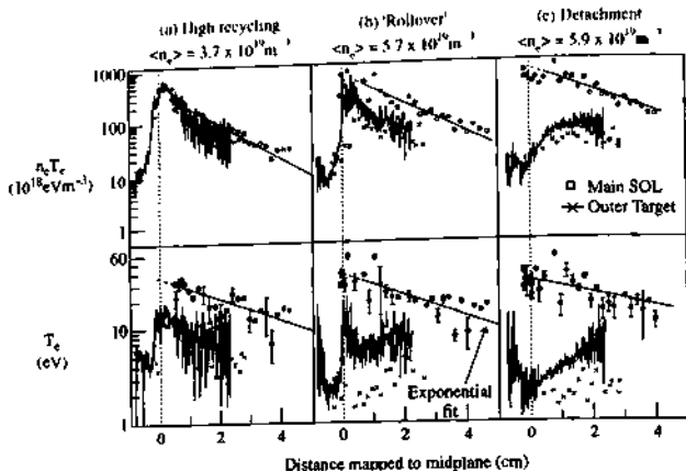
Fig. 12.3.14 Profiles of electron temperature, T_e , and electron pressure, n_e T_e , as a function of distance from the plasma separatrix mapped to the plasma midplane. Three timeslices are shown during an L-mode density ramp: (a) the 'high recycling' attached phase; (b) the 'rollover' as detachment is initiated close to the separatrix; (c) the detached phase. In each case a comparison is made between Langmuir probe measurements made in the SOL close to the plasma midplane and Langmuir probe measurements at the outer divertor target, illustrating the significant fall in temperature at the divertor associated with detachment, together with the substantial pressure drop which develops along the SOL from the midplane to the target [from Loarte, A. et al , Nuclear Fusion 38, 331 (1998)].
