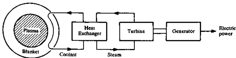
Fig. 1.7.2 Thermuclear power absorbed in blanket would be converted into electric power by conventional means.
