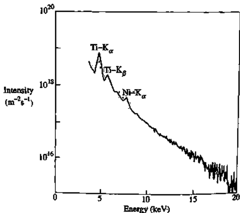
Fig. 10.7.6 X-ray pulse height spectrum for an ohmically heated discharge in JT60. (Kubo, H., et al. Nuclear Fusion 29, 571 (1989).)
