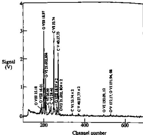
Fig. 10.7.5 UV spectrum in the 5–500 Å region taken on JT60 with a multichannel spectrometer during a discharge with 19 MW of beam heating. (Kubo, H., et al. Nuclear Fusion 29, 571 (1989).)
