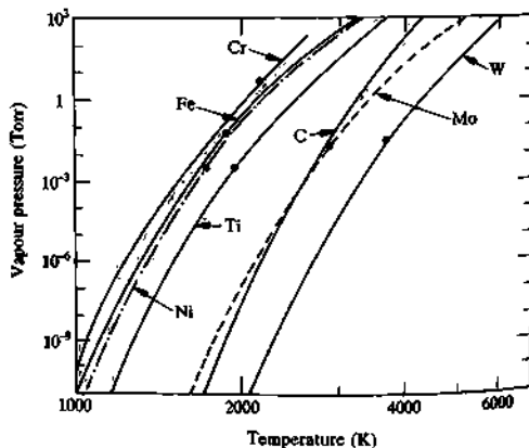
Fig. 9.11.1 Vapour pressure of a range of first wall materials as a function of surface temperature. (Horig, R.E., and Kramer, D.A., Vapour pressure data for the solid and liquid elements. RCA Review 30, 285 (1969).)
