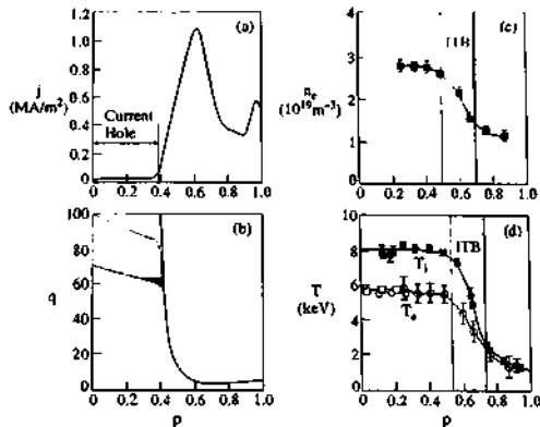
Fig. 12.4.9 Radial profiles of plasma parameters from a plasma with zero current density over the region r/a \leq 0.4 : (a) plasma current density, j , (b) safety factor, q , for which the shaded band indicates the experimental uncertainties, (c) electron density, n_e , (d) ion and electron temperatures, T_i and T_e , respectively [Fujita, T. et al. Physical Review Letters 87 , 245001 (2001)].
