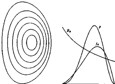
Fig. 3.3.1 Equilibrium flux surfaces and plots of toroidal current density, plasma pressure, and toroidal magnetic field across the midplane.
