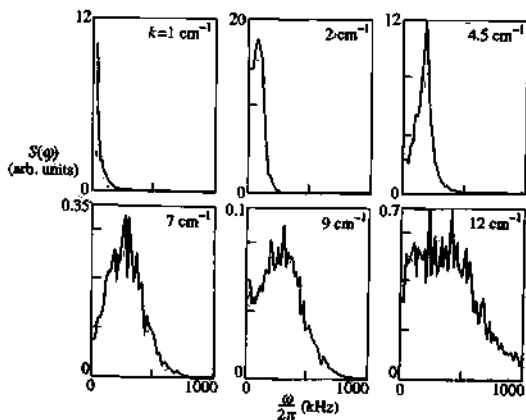
Fig. 10.10.4 Scattered frequency spectra for different values of k . The spectra peak at gradually increasing values of \omega as k increases. (Ritz, Ch.P., Brower, D.L., Rhodes, T.L., Beagerson, R.D., et al. , Nuclear Fusion 27, 1125 (1987).)
