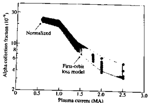
Fig. 12.2.15 \alpha -particle loss fraction captured by a lost \alpha -particle detector located in the bottom of the vacuum vessel, that is in the direction of the ion \nabla B drift. The first orbit loss falls with increasing plasma current in the manner predicted by model calculations. Note that the calculations are normalized to the experimental results at 0.5 MA (Hawryluk, R.J. et al. Plasma Physics and Controlled Nuclear Fusion Research 1994 (Proc. 15th Int. Conf., Seville, 1994) Vol. 1, I). I.A.E.A., Vienna (1995)].
