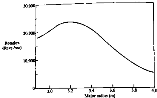
Fig. 3.13.2 Typical radial profile of toroidal rotation of a plasma spun by neutral beam injection (JET).
