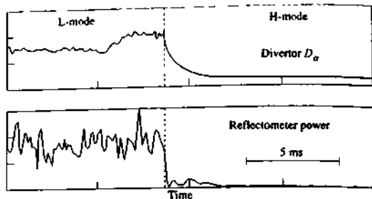
Fig. 4.17.3 Showing the fall of density fluctuations as measured by reflectometry during an L-H transition in DIII-D (Doyle, E.J. et al Plasma Physics and Controlled Nuclear Fusion Research, (Proc. 14th Int. Conf. Würzburg, 1992) Vol. 1, p. 235 I.A.E.A. Vienna (1993))
