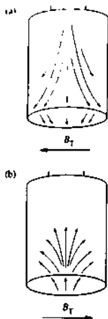
Fig. 9.8.1 Schematic representation of arc tracks observed on curved surfaces of a cylindrical probe exposed in the tokamak boundary. The direction of the arc depends to the direction of the magnetic field.
