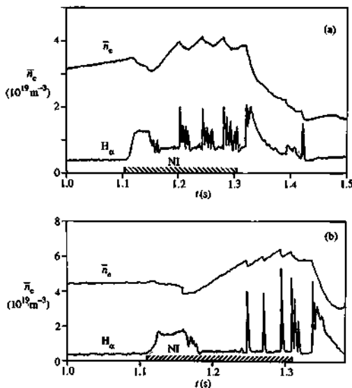
Fig. 7.17.1 H_{\alpha} emission showing ELM activity during H-modes with neutral beam injection in ASDEX, (a) with continuous bursts, and (b) with separated large ELMs. The figure also shows the response of the electron density. (ASDEX Team, Nuclear Fusion 29, 1959 (1989).)
