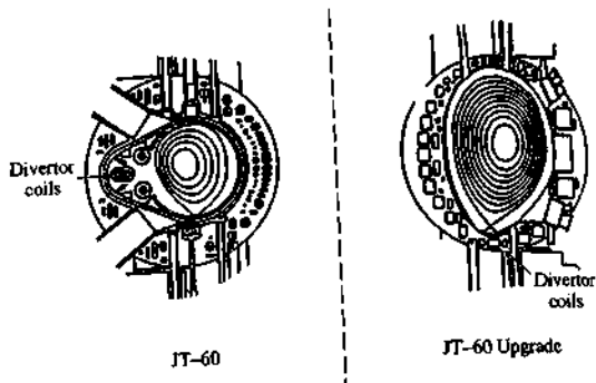
Fig. 12.4.1 Comparison of the final layout of the JT-60 tokamak (left hand side) with the JT-60U (Upgrade) geometry. Note the original triplet of divertor coils at the large major radius side of JT-60 (from JT-60 Team (presented by M. Nagami) Plasma Physics and Controlled Nuclear Fusion Research 1990 (Proc. 13th Int. Conf., Washington, 1990) Vol 1, 53. I.A.E.A., Vienna (1991)).
