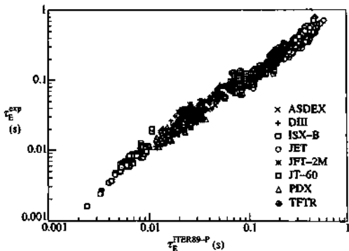
Fig. 4.12.2 Comparison of the experimental values of confinement time from a number of tokamaks with the L-mode scaling \tau_E^{\text{ITER89-P}} . (Yushmanov, P.N. et al. Nuclear Fusion 30, 1999 (1990).)
