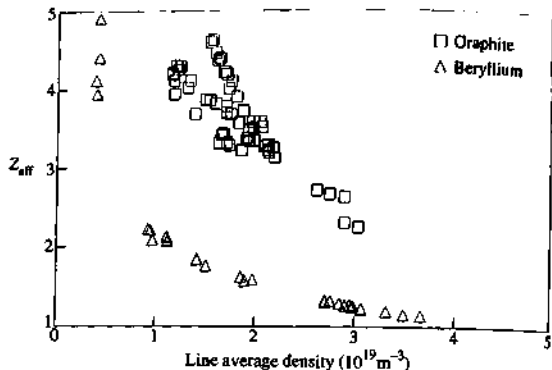
Fig. 12.3.13 Z_{\text{eff}} as a function of density for ohmic discharges using either graphite or beryllium limiters (from The JET Team (presented by K.J. Dietz) Plasma Physics and Controlled Fusion 32, 837 (1990)).
