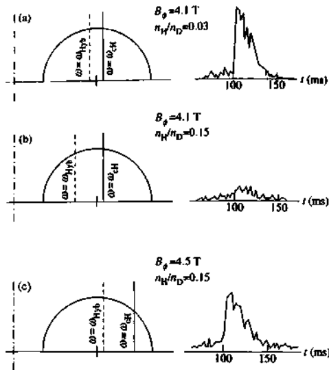
Fig. 5.8.4 Effect of n_H/n_D on the neutron rate at different values of the magnetic field in 'low density' plasmas. Strong absorption (high count) only occurs when the ion-ion hybrid resonance is at the centre of the discharge. [Adam J. and Equipe TFR., Proceedings of 9th European Conference on Controlled Fusion and Plasma Physics , Oxford 1979, Invited Papers, UKAEA Culham Laboratory, p. 355.]
