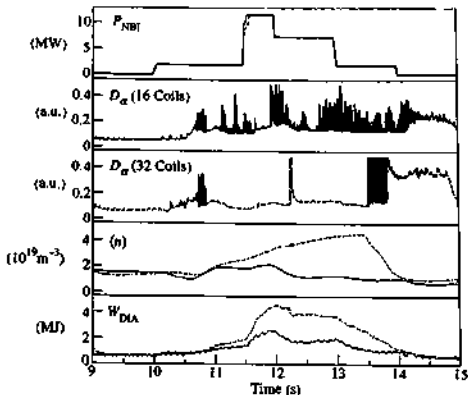
Fig. 12.3.12 Comparison of NBI H-modes with 16 coils (high toroidal field ripple—solid traces) and 32 coils (low toroidal field ripple—dashed traces). Shown are NBI power, P_{\text{NBI}} , D_{\alpha} emission signals for 16 and 32 coil cases, volume averaged density, \langle n \rangle , and stored energy from diamagnetic measurements, W_{\text{DIA}} [The JET Team (presented by B.J.D. Tubbing) Plasma Physics and Controlled Nuclear Fusion Research 1992 (Proc. 14th Int. Conf., Würzburg, 1992); Vol 1, 429. I.A.E.A., Vienna (1993)].
