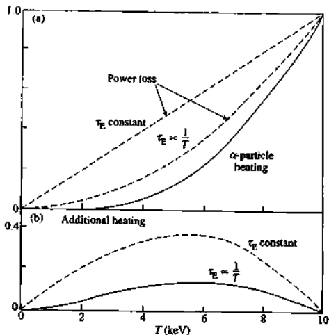
Fig. 5.1.1 Showing the power balance for a tokamak which would ignite at a temperature of 10 keV. Figure (a) gives the rate of power loss per unit volume for \tau_E = \text{constant} and \tau_E \propto 1/T , together with the corresponding \alpha -particle heating. Figure (b) gives the additional heating per unit volume to provide a steady state power balance in the two cases. The powers are normalized to the \alpha -particle heating (and therefore to the power loss) at ignition.
