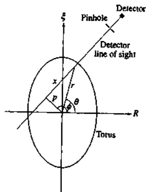
Fig. 10.8.5 Geometry of detectors for tomographic inversion. The relationship is shown between the plasma coordinates (r, \theta) and the detector's coordinates (p, \phi) .
