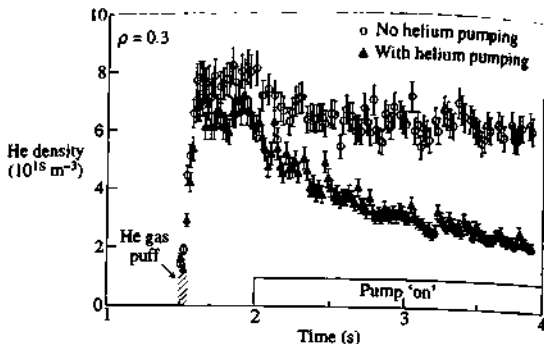
Fig. 12.5.16 Helium density at \rho = 0.3 , as measured by active CXRS, as a function of time for discharges with and without active helium pumping. A short, 50 ms, helium puff is injected at 1.5 s and the pumping is 'switched on' at 2 s by changing the radial position of the outer divertor strike point. In the case with active helium pumping, provided by argon frosting of the cryopump, the helium concentration of the core plasma decays on a timescale of \sim 1 s [Hillis, D.L. et al. Plasma Physics and Controlled Fusion 36, A171 (1994)].
