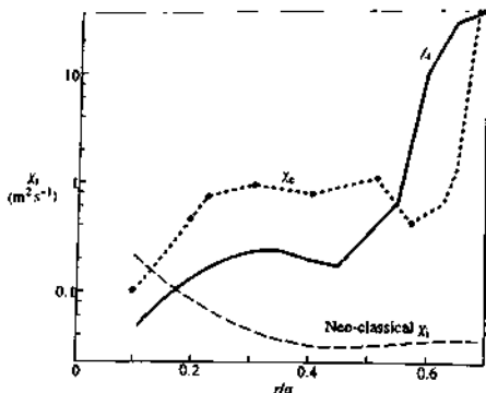
Fig. 4.14.1 Radial profiles of the ion, electron and neoclassical diffusivities for an optimized shear D-T discharge in JET. (JET Team, Nuclear Fusion 39, 1 (1999).)
