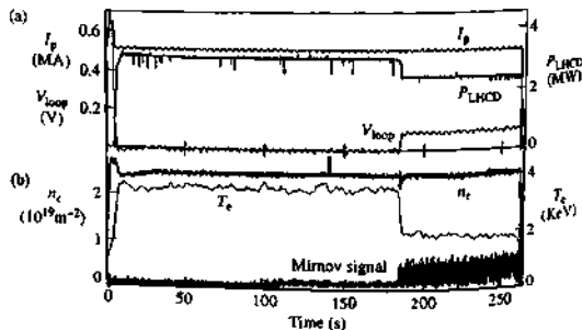
Fig. 11.16.1 Tore-Supra discharge with a duration of 4 min 25 s in which 0.75 GJ was exhausted from the plasma. Time evolution of (a) plasma current, loop voltage, and LHCD power (b) central line integrated density, electron temperature at normalized radius 0.3 and the Mirnov coil signal.
