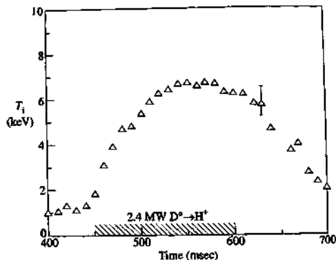
Fig. 5.4.6 Heating of PLT plasma by neutral beam injection. The ion temperature was measured by analysis of charge-exchange neutrals for 2.4 MW deuterium injection into a plasma with a central density n(0) = 4.5 \times 10^{19} \text{ m}^{-3} . (Eubank, H. et al. Physical Review Letters 43, 270 (1979).)
