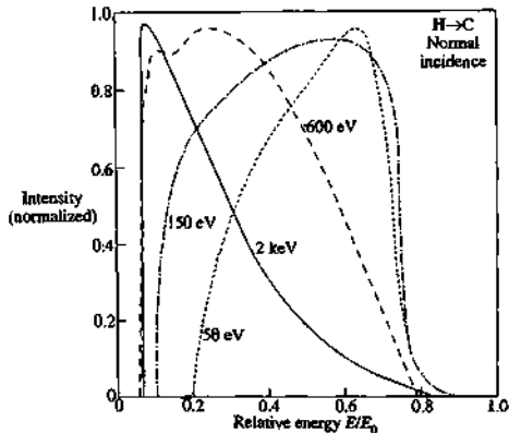
Fig. 9.4.2 Measured energy distribution of hydrogen atoms backscattered from carbon, for different incident ion energies, E_p . The distributions are normalized at their maximum intensity. (Azari, R. and Eckstein, W., J Nuclear Materials 910, 162-4 (1989).)
