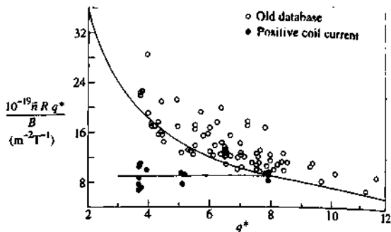
Fig. 12.5.10 Plot of the lower limit of the operating region which is stable against locked n = 1 modes induced by error fields in the 10^{-19} \bar{n} R q^* / B vs q^* plane. The open circles represent points from experiments without an error field correction system, with the upper line illustrating the operating boundary q^* D = 72 \text{ m}^{-2} \text{ T}^{-1} , where D = 10^{-19} \bar{n} R q^* / B . The solid circles correspond to experiments using a simple n = 1 correction coil and the lower line shows the improved operating boundary D = 9 \text{ m}^{-2} \text{ T}^{-1} [Scoville, J.T. et al. Nuclear Fusion 31, 875 (1991)].
