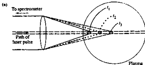
Fig. 10.5.3 (a) The principle of LIDAR is shown. The very short laser pulse successively illuminates different parts of the plasma at r_1, r_2, r_3 . (b) The dispersed signals of the scattered radiation at three different wavelengths as a function of time, or equivalently, major radius. (c) Electron density and temperature profiles deduced from the scattered spectra at different times. The considerable rise in n_e and T_e was a consequence of the 13.5 MW of additional heating which was applied at 6 s.
