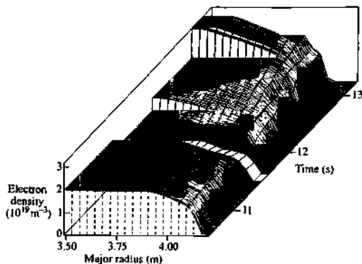
Fig. 10.4.2 Electron density profiles measured with the multiple frequency, narrow band sweep system on JET. In the flat regions no measurements were made
