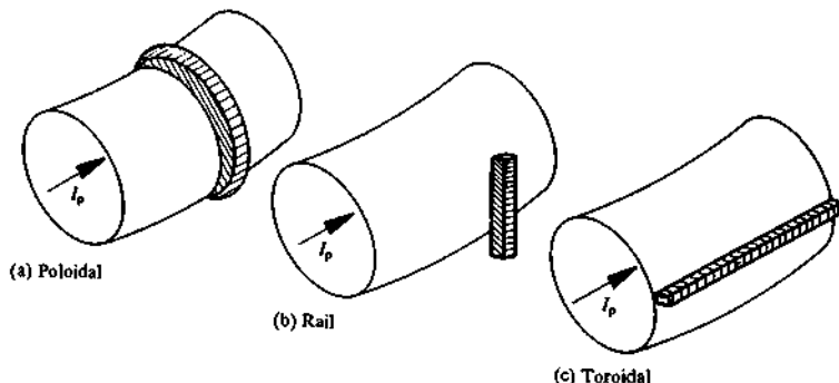
Fig. 9.9.1 Schematic representation of different types of limiter.
