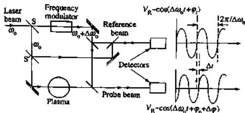
Fig. 10.3.1 Schematic layout of a Mach-Zehnder interferometer. The laser beam is split at S and S' and recombined at the detectors. The phase differences \phi_p and \phi_r reflect the different path lengths whereas \Delta\phi is caused by the refractive effects of the plasma only.
