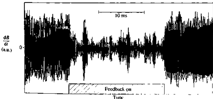
Fig. 11.7.1 Showing the reduction in the m = 2 component of the magnetic field fluctuations in DITE on the application of feedback control. The bursts of increased signal during the stabilized period are coincident with sawteeth.
