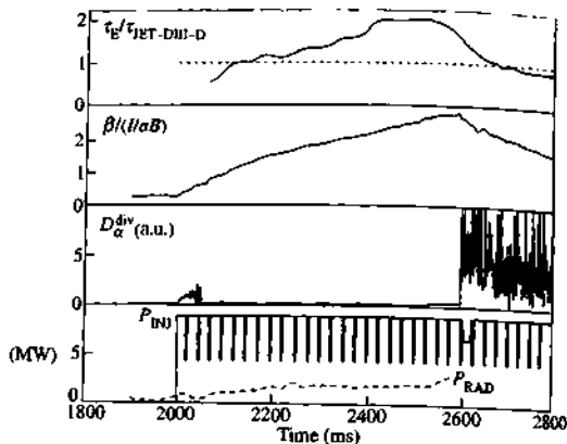
Fig. 12.5.5 Typical waveforms for a VH-mode discharge. The ratio of the thermal energy confinement time to the JET/DIII-D scaling expression, \tau_E/\tau_{JET-DIII-D} , increases to \sim 2 during the VH-mode. Also shown are the normalized toroidal beta, \beta/(I/aB) , the divertor D_\alpha emission, the injected NBI power, P_{INJ} , and the radiated power, P_{RAD} (from DIII-D Team (presented by R. D. Stambaugh) Plasma Physics and Controlled Nuclear Fusion Research 1994 (Proc. 15th Int. Conf., Seville, 1994) Vol 1, 83. I.A.E.A., Vienna (1995)).
