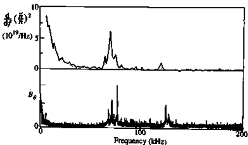
Fig. 7.15.4 Spectrum of TAE density fluctuations as measured by beam emission spectroscopy on TFTR together with that of the magnetic fluctuations, \delta B , measured by a Mirnov coil. (Wong, K.L. et al. , Physical Review Letters 66, 1874 (1991).)
