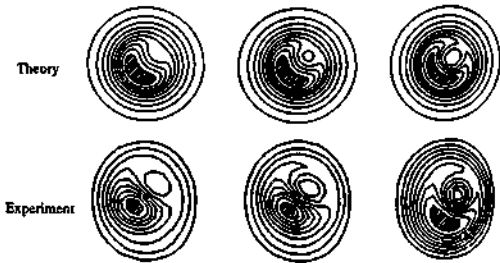
Fig. 7.6.9 Comparison of a quasi-interchange simulation (P. Kirby) with the deformation as reconstructed from the soft X-ray emission on JET (R. Granetz).
