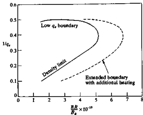
Fig. 7.8.1 Typical Hegill diagram showing the operating regime as limited by disruptions. q_0 is the safety factor at the surface of the plasma and \bar{n} the mean electron density. The parameter 10^{-19} \bar{n} R / B_0 is called the Murakami parameter.
