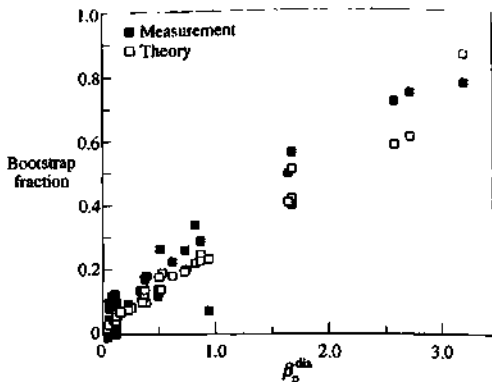
Fig. 12.4.8 Bootstrap current fraction as a function of \beta_p^{dia} , showing both measured values and values derived from neoclassical theory including the bootstrap current contribution [Ishida, S. et al. Plasma Physics and Controlled Nuclear Fusion Research 1990 (Proc. 13th Int. Conf., Washington, 1990) Vol 1, 195. I.A.E.A., Vienna (1991)].
