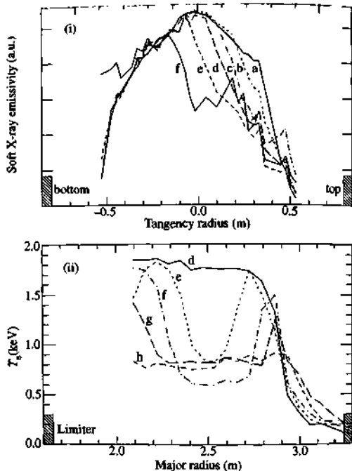
Fig. 12.2.8 (i) Vertical profiles of chord integrated soft X-ray emissivity showing the downward penetration, at this toroidal location, of an m = 1 deformation of the plasma core. (ii) Profiles of electron temperature, derived from ECE measurements in the horizontal midplane, showing the m = 1 deformation appearing as a 'cold bubble'. Profiles are taken at 50 \mu\text{s} intervals during the last 500 \mu\text{s} before the thermal quench [Fredrickson, E.D. et al. Nuclear Fusion 33, (4) (1993)].
