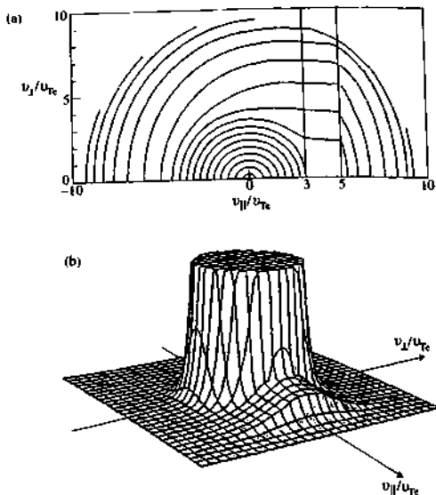
Fig. 5.9.3 Contours of steady state electron distribution in (v_{\perp}, v_{\parallel}) space for lower hybrid current drive. (a) represents contours of constant f(v_{\perp}, v_{\parallel}) where v_{\perp} and v_{\parallel} have been normalized to v_{Te} and (b) shows the surface f(v_{\perp}, v_{\parallel}) truncated at 0.02 times the maximum in f , in order to show the plateau more clearly. [From Karney, C.F.F. and Fisch, N.J., Physics of Fluids 22, 1817 (1979).]
