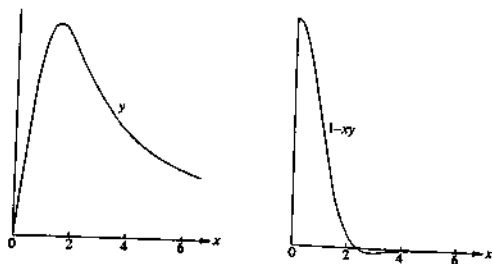
Fig. 6.8.2 Solutions for y and (1-y) across the resistive layer.
