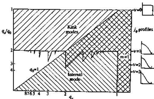
Fig. 6.10.4 Kink stability diagram (Fig. 6.7.2) with inclusion of internal kink stability boundary.
