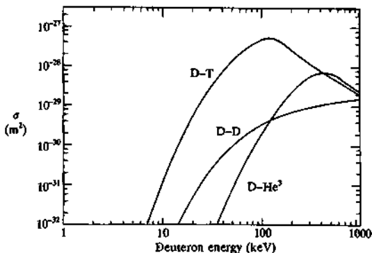
Fig. 1.2.2 Cross-sections for the reactions D-T, D-D and D-He 3 . The two D-D reactions have similar cross-sections, the graph gives their sum.
