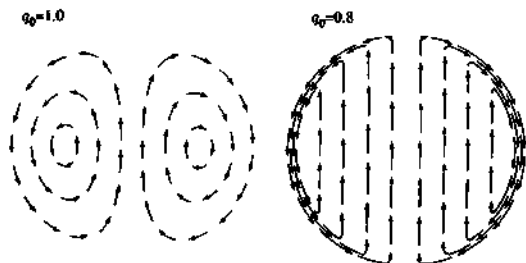
Fig. 6.10.3 Flow pattern of quasi-interchange ( q_0 = 1.0 ) and rigid shift ( q_0 = 0.8 ).
