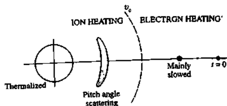
Fig. 5.4.4 Sketch of the time development of the velocity distribution of beam ions injected at t = 0 , showing the change in behaviour when the ions are slowed below the critical velocity v_c = (2kT_e/m_b)^{1/2} .
