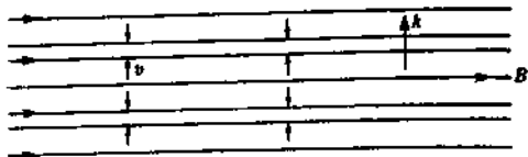
Fig. 2.24.4 The fast magnetosonic with k \perp B_0 . The oscillations involve compression of both the fluid and the magnetic field.
