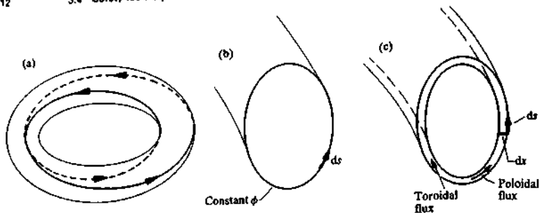
Fig. 3.4.1 (a) Field lines on q = 2 surface. (b) Poloidal integration path for eqn 3.4.2. (c) Flux annulus containing toroidal flux d\Phi and poloidal flux d\Psi .
