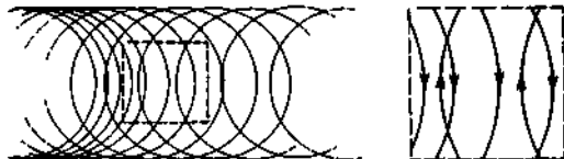
Fig. 2.22.2 Showing how a density gradient of stationary orbits give rise to a local current. The current arises through a local imbalance of upward and downward moving particles as illustrated in the enlarged section.
