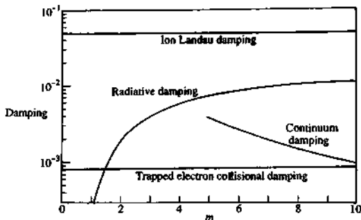
Fig. 7.15.3 Graphs showing the m -dependence of the contributions to the normalized damping rate of TAE modes for an ITER equilibrium (from Connor, J.W. et al. , Proc. 21st European Phys. Soc. Conf. on Controlled Fusion and Plasma Physics, Montpellier 1994).
