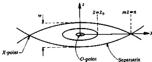
Fig. 7.2.2 Geometry of magnetic field lines of a magnetic island in the (z, \chi) plane.
