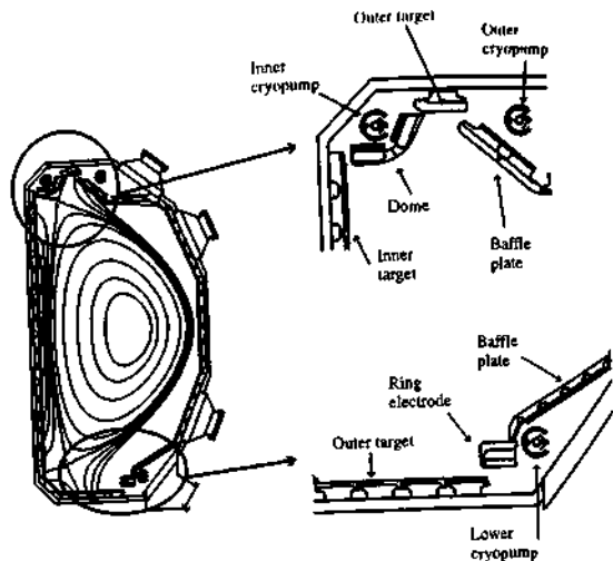
Fig. 12.5.2 Cross-section of the DIII-D vacuum vessel showing the main elements of the upper and lower pumped divertors.
