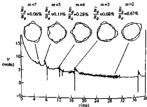
Fig. 10.2.3 The evolution of the loop voltage trace and observed structure of magnetic perturbations during the current rise in Alcator A. (Granetz, R.S. et al. , Nuclear Fusion 19, 1587 (1979).)
