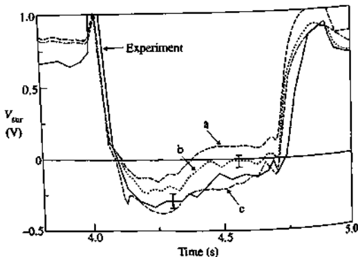
Fig. 12.2.7 The time variation of the surface loop voltage, V_{\text{star}} , determined experimentally from magnetic measurements, shown by the solid line, and calculated under various assumptions: (a) ohmic current only, (b) NBI-driven and ohmic currents, and (c) bootstrap, NBI-driven, and ohmic currents [Zarnstorff, M.C. et al. Physical Review Letters 60 , 1306 (1988)].
