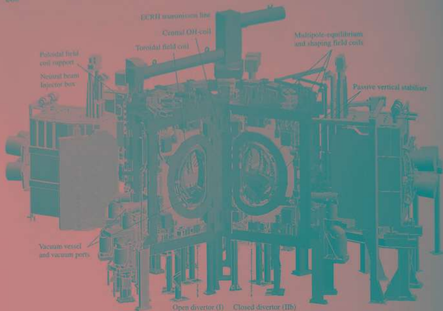
Fig. 12.6.1 3D cut away view of ASDEX Upgrade with neutral beam injector boxes and DIV I (left) and DIV IIb (right) divertor configuration.
