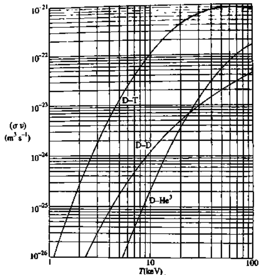
Fig. 1.3.3 \langle \sigma v \rangle for D-D (total) and D-He 3 reactions as a function of plasma temperature. The values are much smaller than those for D-T which are included for comparison.
