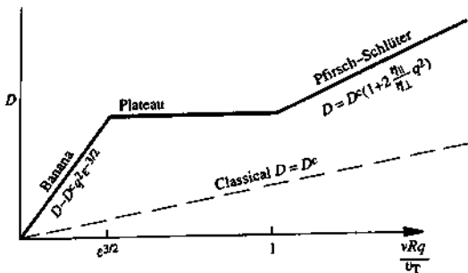
Fig. 4.7.1 Variation of diffusion coefficient with collision frequency.
