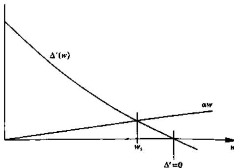
Fig. 7.3.1 Plots of \Delta'(w) and \alpha w , which determine the growth and saturation of tearing mode magnetic islands.
