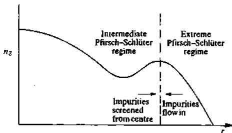
Fig. 4.22.1 Predicted neoclassical impurity fluxes near plasma edge, showing impurity accumulation.
