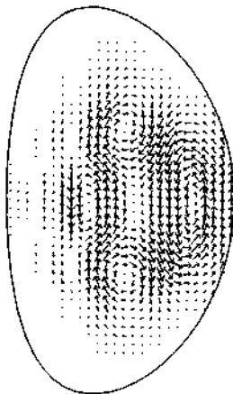
Fig. 6.4.1 Showing the poloidal component of the displacement \xi for an ideal mhd instability in a tokamak.
