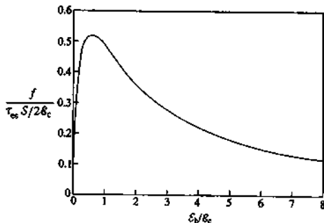
Fig. 5.4.3 Graph of the steady state energy distribution function resulting from the slowing-down of an ion beam.
