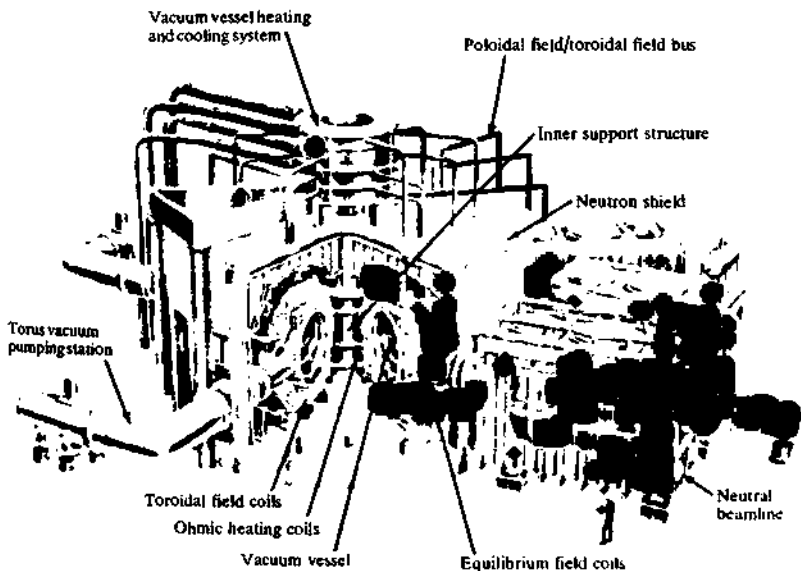
Fig. 12.2.1 Layout of the TFTR experiment.
