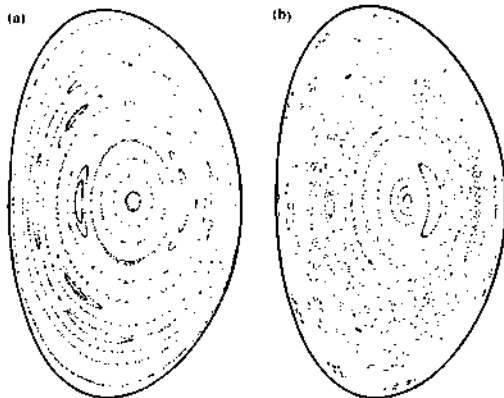
Fig. 7.13.2 Calculated intersections of magnetic field lines with a chosen poloidal plane in a tokamak. In (a) mhd perturbations produce magnetic islands and in (b) a higher level of perturbation leads to a substantial region of ergodic behaviour.
