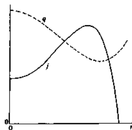
Fig. 7.5.1 Skin current profile and associated q -profile.
