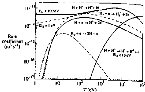
Fig. 9.5.1 Rate coefficients for hydrogen atoms and molecules for a number of common reactions. The first symbol refers to the test particle and the second refers to the thermal species, the rate coefficient being integrated over the Maxwellian distribution of this species. E_H is the energy of the test particle (R.K. Janev et al. Elementary processes in hydrogen-helium plasmas, cross sections and reaction rate coefficients , Springer-Verlag, Berlin, 1987).
