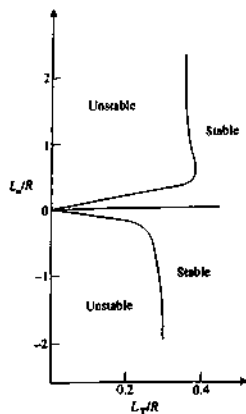
Fig. 8.3.3 Stability diagram for the toroidal ITG mode (from Biglari H. , et al. , Physics of Plasmas B1 109 (1989)).
