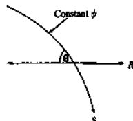
Fig. 3.13.3 Geometry used in the calculation of centrifugal effects.
