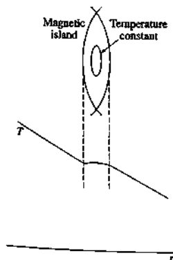
Fig. 7.9.4 The temperature across the midplane of a magnetic island is flattened through the equalization of the temperature around the interior flux surfaces.
