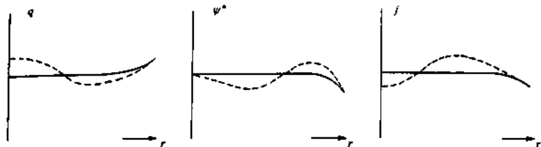
Fig. 7.5.3 Graphs of q(r) , \psi^*(r) , and j(r) before the instability (dashed lines) and after the instability (full lines). The instability flattens q and enhances the current penetration.
