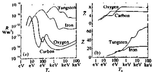
Fig. 4.25.1 (a) The radiation parameter R and (b) the mean charge \bar{Z} as functions of electron temperature for carbon, oxygen, iron, and tungsten.
