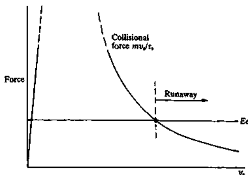
Fig. 2.17.1 The electric field force, Ee , and the collisional force for an electron with a velocity v_e .
