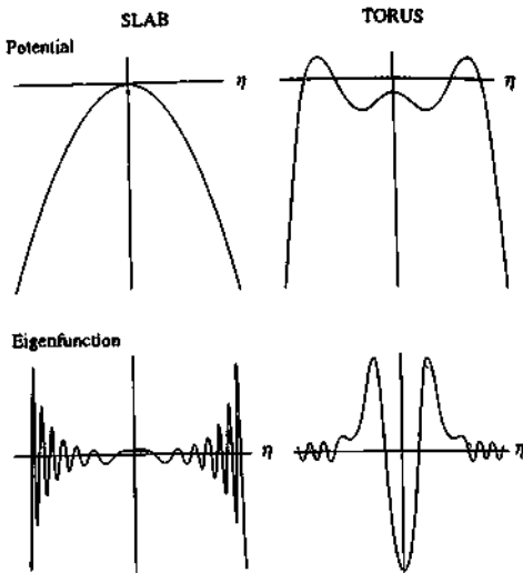
Fig. 8.3.2 Plots showing the 'potential' for the electron drift mode and the corresponding eigenfunction as a function of the ballooning coordinate \eta , for the toroidal coupling parameter \alpha = 0 (left) and \alpha = 3 (right).
