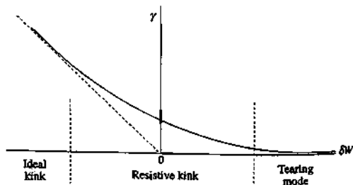
Fig. 6.11.1 Schematic graph of the dependence of the growth rate of the m = 1 mode on \delta W , illustrating the transition from the ideal kink ( \delta W < 0 ) to the tearing mode ( \delta W > 0 ) through the resistive kink mode.
