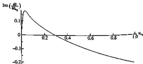
Fig. 8.4.2 Variation of growth rate with electron collisionality, \nu_e/\epsilon , for the trapped ion mode where \nu_i = (m_e/2m_i)^{1/2} \nu_e is assumed and the other parameters are fixed.
