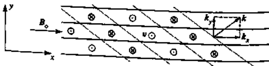
Fig. 2.24.2 General shear Alfvén wave. \mathbf{B}_0 and \mathbf{k} lie in the plane of the figure and the velocity oscillation is perpendicular to this plane. The wave propagates along x with the Alfvén velocity V_A .
