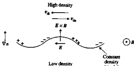
Fig. 8.4.1 The physical mechanism for the trapped particle instability. The charge polarization caused by the curvature drift of the trapped particles results in an \mathbf{E} \times \mathbf{B} flow which enhances the amplitude of an initial density wave and results in instability.
