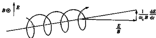
Fig. 2.6.4 Polarization drift of an ion caused by an increasing electric field perpendicular to the magnetic field. The electrons drift in the opposite direction.
