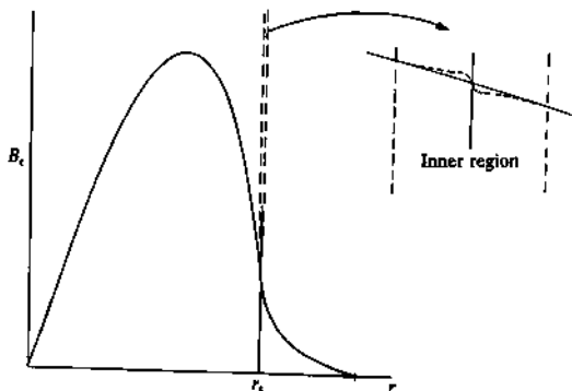
Fig. 6.8.1 Showing a typical form of B_1(r) . The full line in the expanded view of the inner region is the actual (resistive) solution. The dashed line shows the continuation of the outer (ideal) solution.
