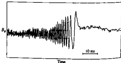
Fig. 7.10.1 The magnetic signal B_\theta shows the frequency and growth of an n = 1 tearing mode. The reduction in frequency corresponds to a fall of the propagation speed, and the removal of the gross oscillation indicates the final mode locking (JET).
