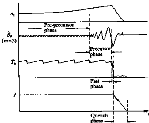
Fig. 7.7.2 Showing typical time dependence of the m = 2 magnetic fluctuations, central temperature, and plasma current during the period of a disruption. In this example the disruption is precipitated by a density increase as shown.
