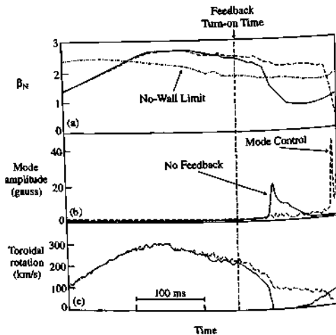
Fig. 12.5.12 Comparison of (a) \beta_N , (b) resistive wall mode amplitude, (c) plasma toroidal rotation for pulses with \beta_N above the no-wall \beta -limit. Two cases are shown, no active feedback control of the resistive wall mode (solid line) and active feedback control using a 'mode control' algorithm (dashed line), illustrating the extension of the pulse duration at high- \beta_N with active magnetic feedback [from Garofalo, A.M. et al. Fusion Energy 2000 (Proc. 18th Int. Conf., Sorrento, 2000) paper IAEA-CN-77/EXP3/01(R), I.A.E.A., Vienna (2001)].
