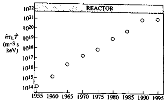
Fig. 1.1.1 In a reactor the product n\tau_E of ion density and energy confinement time, and the temperature, T , must both be in the right range. Taking peak values, the required n\tau_E is 2-5 \times 10^{20} \text{ m}^{-3} \text{ s} and the temperature range is around 10–20 keV. The required value of the product \hat{n}\tau_E\hat{T} is approximately 5 \times 10^{21} \text{ m}^{-3} \text{ s keV} (Section 5.1). The figure shows the progress in improving this product, leading to the verge of reactor conditions.
