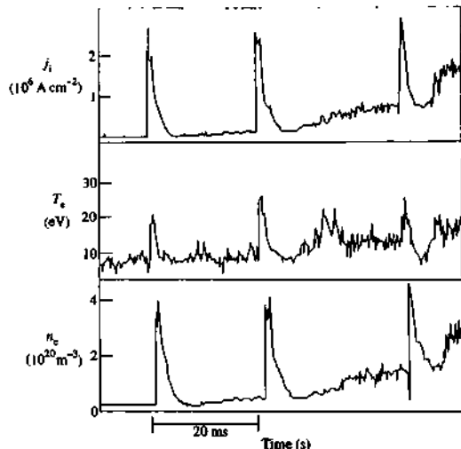
Fig. 10.9.4 Divertor triple probe data from an ELMy discharge in JET.
