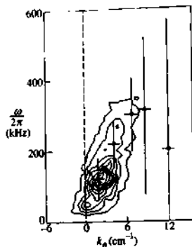
Fig. 10.10.5 S_s(\theta, \omega) spectrum at r = 0.26 m in TEXT from scattering experiments (crosses which represent FWHM) and from Langmuir probe measurements (contours). (Woodson, A.J., Austin, M.E., Bengtson, R.D., Boedo, J.A., et al. FRCR#310, University of Texas, Austin (1998).)
