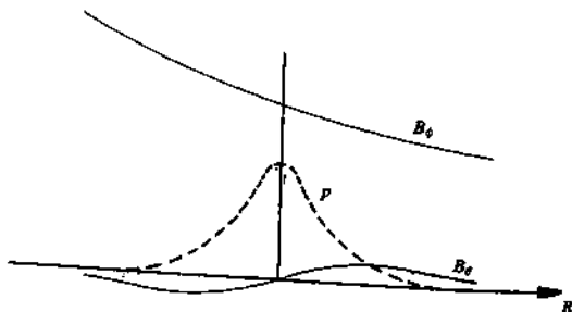
Fig. 3.1.1 Basic radial variation of the toroidal magnetic field B_\phi (with an approximate 1/R dependence), the poloidal magnetic field B_\theta , due mainly to the plasma current, and the plasma pressure, p . R is the distance from the major axis of the torus and the graphs are for the median plane.
