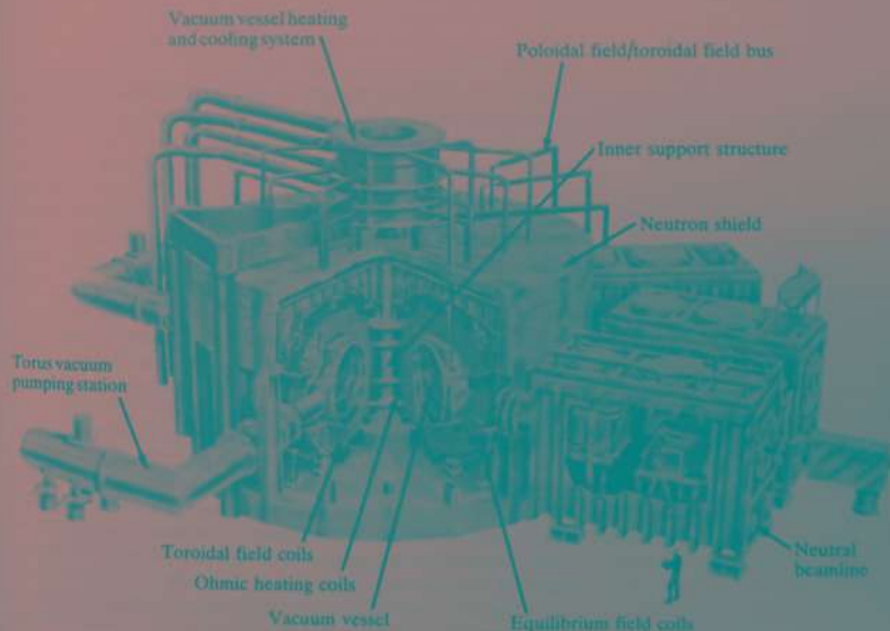
Fig. 12.2.1 Layout of the TFTR experiment.
