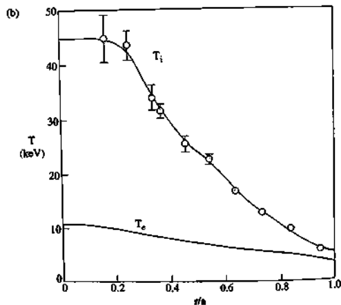
Fig. 12.4.13 Overview of the high- \beta_p H-mode with the highest fusion triple product. Shown are: (a) the diamagnetic stored energy, W_{dia} , the absorbed heating power, P_{abs} , the neutron emission, S_n , the edge ion temperature, T_i(0.94a) , the line-averaged electron density, \bar{n}_e , along chords at r/a = 0 and r/a = 0.76 , the energy confinement time, \tau_E , the D_p emission from the divertor region, D_p^{div} , and the signal from a saddle coil system for detecting mhd modes with n = 2 ; (b) the radial ion and electron temperature profiles, T_i and T_e respectively, at the time of peak fusion performance [from Ishida, S. et al. Fusion Energy 1996 (Proc. 16th Int. Conf., Montreal, 1996) Vol 1, 315. I.A.E.A., Vienna (1997)].
