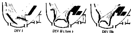
Fig. 12.6.2 Evolution of divertor configurations in ASDEX Upgrade: DIV I (1991-1997), DIV II (1997-2000), DIV IIb adapted to higher triangularity plasmas
