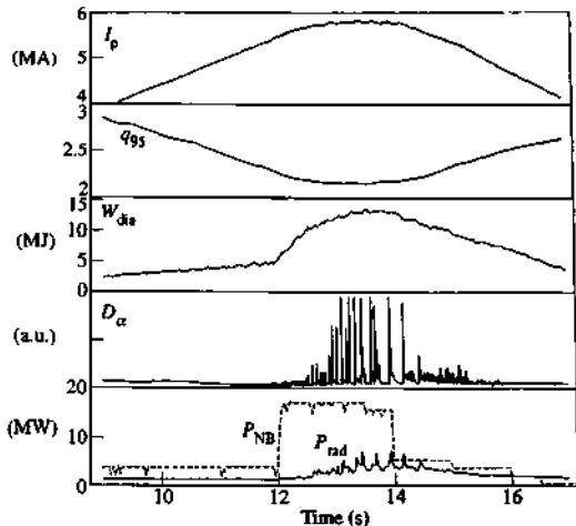
Fig. 12.3.10 Parameters of a JET 6 MA H-mode showing the plasma current, I_p , the safety factor at the 95% flux surface, q_{95} , the plasma diamagnetic energy, W_{dis} , the D_\alpha emission, the neutral beam power, P_{NB} , and the radiated power, P_{rad} .
